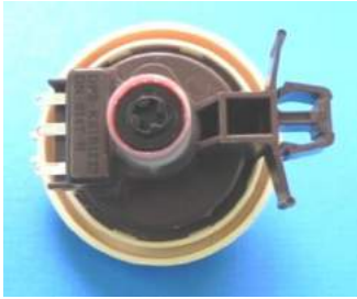
Pressure Sensor (S Type)
