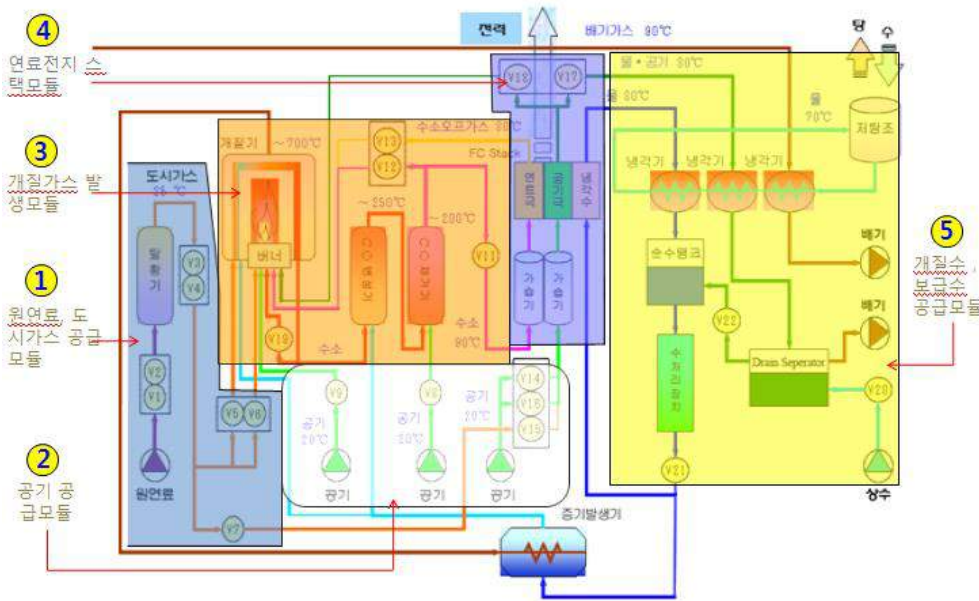
Fuel Cell System (Japan)
